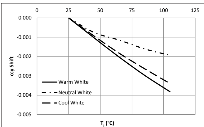
Figure 14: Typical ccy Shift vs. Case Temperature
