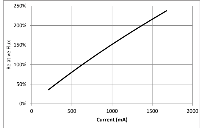
Figure 11: V13C Typical Relative Flux vs. Current ( T_c=25^\circ\text{C} )
