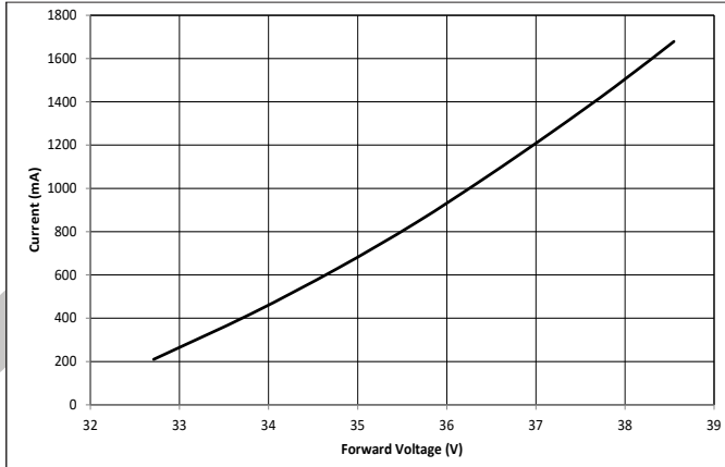
Figure 10: V13C Drive Current vs. Voltage ( T_c=25^\circ\text{C} )
